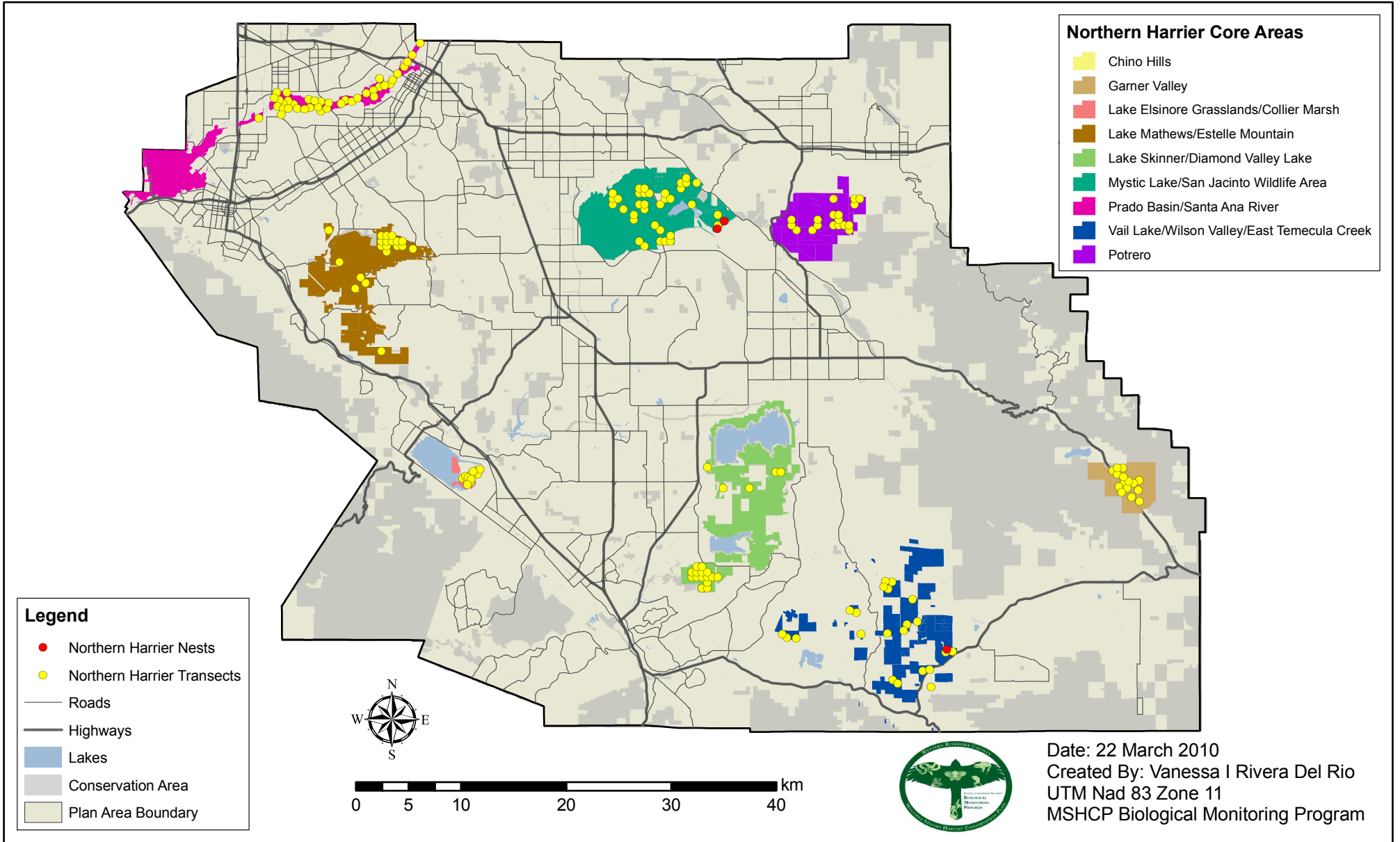
Figure 1. Core Areas, transect midpoints, and nest locations for northern harriers in 2009.
